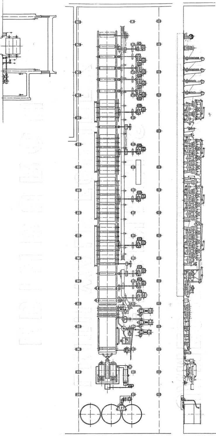
Wire 117 inches wide, 65 feet long with two "Leith Walk" Drum Strainers, Suction Couch, one Suction Press and one plain Press, Wet Smoothers, 29 Drying Cylinders 4 feet 6 inches diameter, Dry Smoothers four Calenders, Coolers, Reeler and Harland Sectional Electric Drive.
